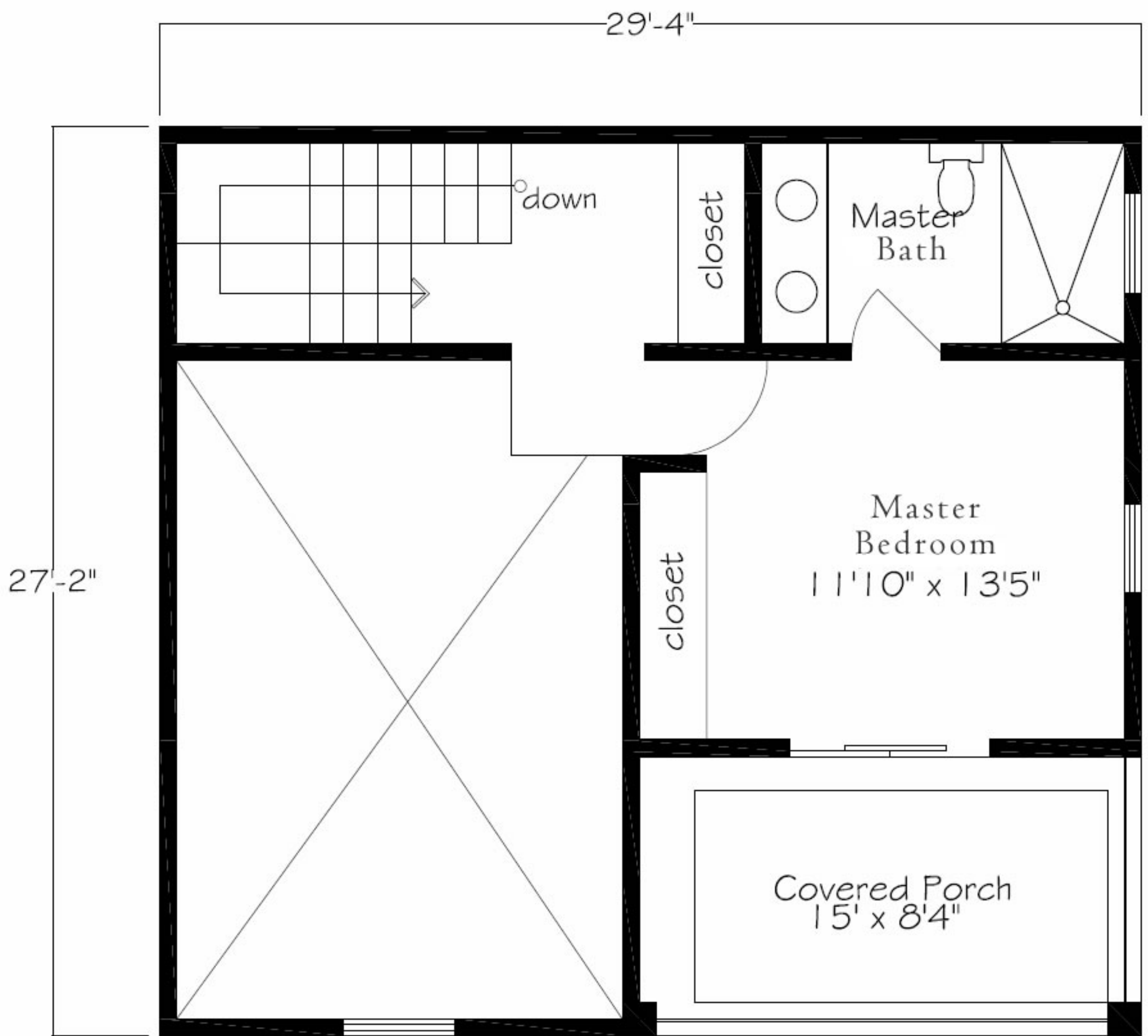
Floor Plan_ 2nd Santo Domingo
